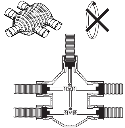
Uponor Ecoflex H-insulation set 200/175/140
