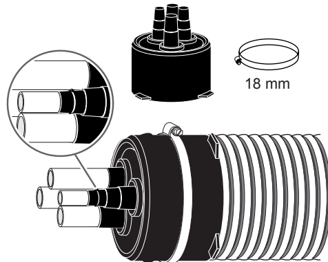
Uponor Ecoflex rubber end cap Quattro 18-28+32+40/200
